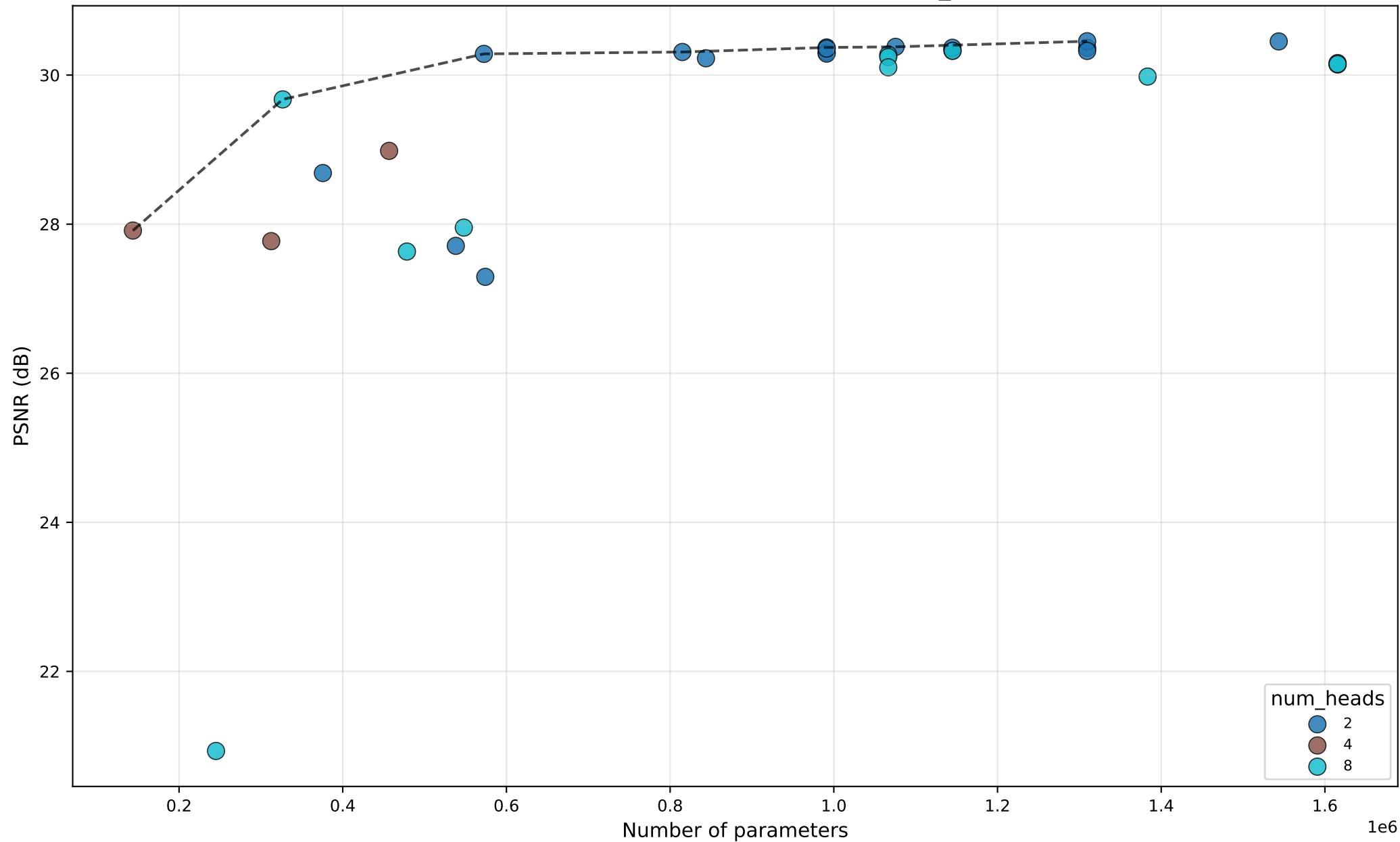
PSNR vs #Params — SRFormer — by num_heads
